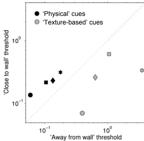
Figure 5. The effect of target location. Thresholds measured when the target square was close to the wall are plotted against thresholds measured when the target was presented in the centre of the room (re-plotted from Figure 4) for a reference distance of 1 m. Black symbols indicate thresholds for detecting a change in the 'physical' distance of the target and grey symbols indicate 'texture-based' thresholds. Symbols for the individual participants correspond to those in Figure 4 and Figure 6.
