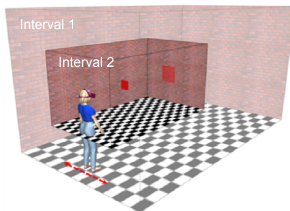
Figure 1. The virtual scene. The semi-transparent and opaque parts of the figure represent the scene in Intervals 1 and 2, respectively. The participants were required to move from side to side to generate motion parallax (red arrow). In a 2IFC task, participants compared the distance to two squares presented in separate intervals.
