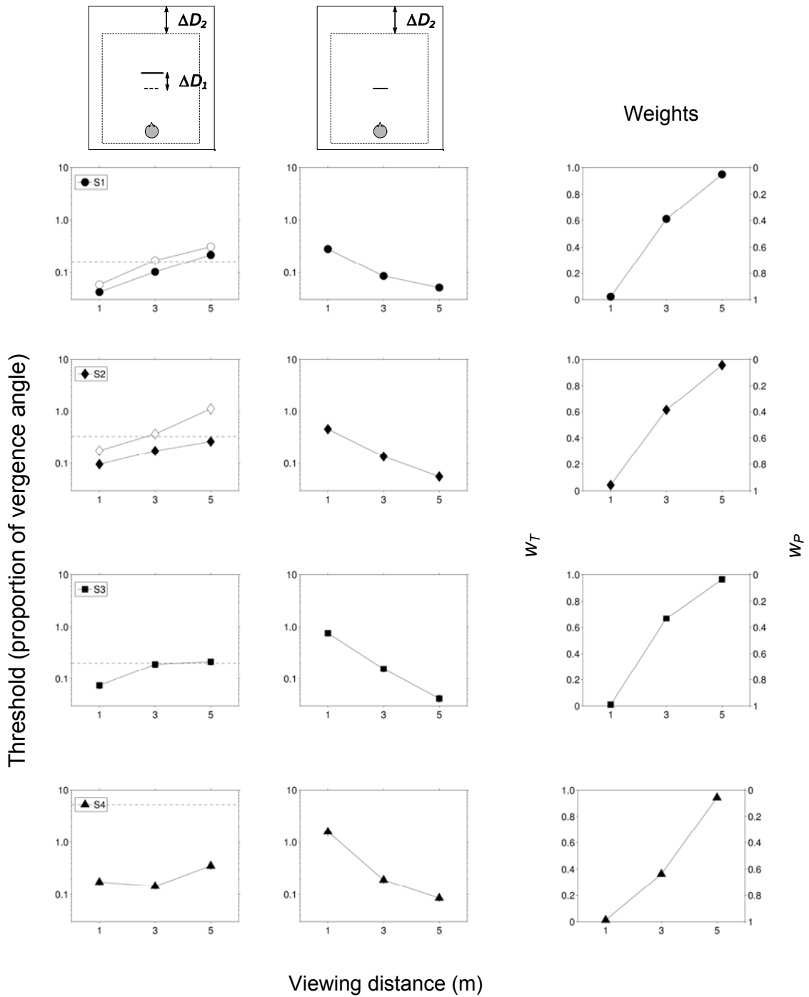
Figure 4. Thresholds for detection of change in ‘physical’ and ‘texture-based’ cues. The first column shows thresholds for detecting a change in distance to the square when there is no change in texture-based cues (referred to as ‘physical’ threshold, see Table 1). The icon above shows the change in distance to the square ( \Delta D_1 ) and the proportional change in the room ( \Delta D_2 for the back wall). Thresholds are given as a Weber fraction defined as a proportional change in the vergence angle compared to fixating the reference square. Closed symbols indicate conditions in which the target was surrounded by the brick room. For two participants, open symbols show data for the target presented on its own. The dashed line shows the threshold for detecting a change in room size alone (without any square). The second column shows thresholds when there was no change in location of the target square between intervals, only a change in its distance relative to the surrounding room (referred to as ‘texture-based’ threshold) as shown in the icon above. The third column shows weights for ‘physical’ and ‘texture-based’ cues derived from these thresholds ( w_P and w_T respectively).
