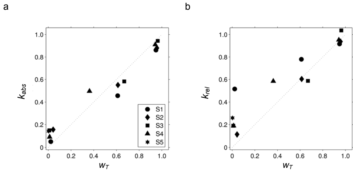
Figure 6. Predictions and fits for distance matching results when the target was in the middle of the room. The fits to the matching data for both tasks ( k_{abs} and k_{rel} , re-plotted from Figure 3b) are plotted against the predicted weight for texture-based cues, w_T (replotted from Figure 4). a) k_{abs} is the weighting determined by a best fit to the matching data when participants judged the perceived absolute distance of the target. b) k_{rel} is the weighting derived from judgements of target distance relative to the room.
