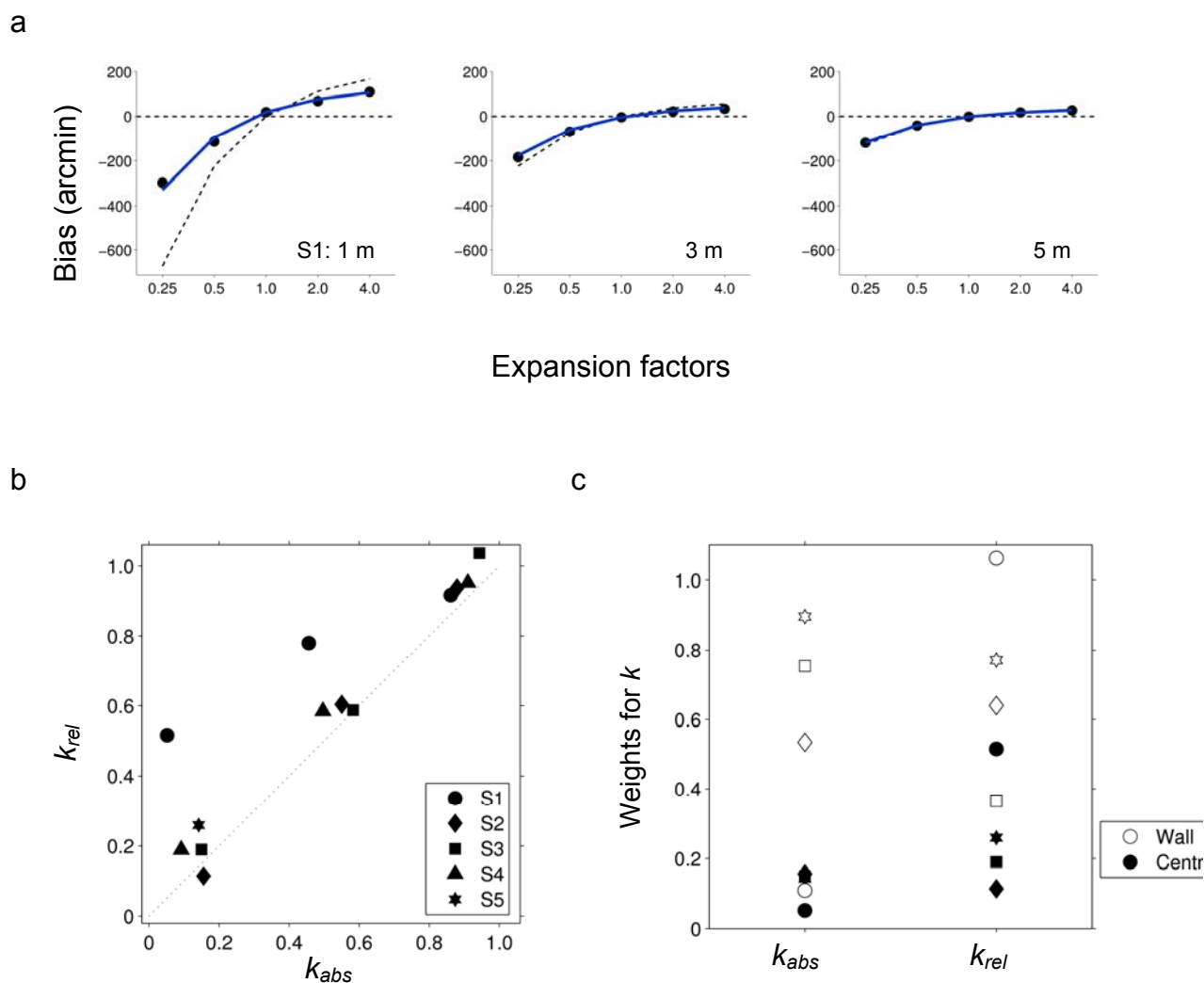
Figure 3. Distance matching from the 'relative' task in Experiment 1. The experiment was the same as for Figure 2, except that participants were asked to judge the distance of the reference and comparison squares in relation to the room. a) Data for the same participant (S1) as shown in Figure 2a. For this participant, the change in task makes a substantial difference to the matches. b) Values of the weighting parameter for the 'relative' task ( k_{rel} ) plotted against those for the 'absolute' task ( k_{abs} ), shown for the four participants in Figure 2 and a fifth participant for a reference distance of 1 m. Participant S1 (circles) is atypical in showing a large effect of task. c) Data for the condition in which reference and comparison squares were presented close to the wall. Open symbols show the weighting parameter k_{abs} derived from the absolute task and k_{rel} for the relative task. Closed symbols show k_{abs} and k_{rel} replotted from b).
