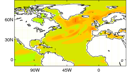
SST sdv ratio (low/total) MAR (GC3.1)
