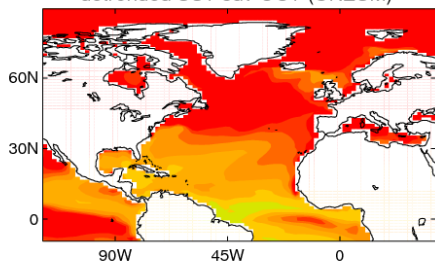
detrended SST sdv OCT (UKESM)
