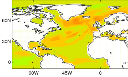
SST sdv ratio (low/total) JAN (GC3.1)
