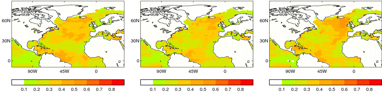
detrended SST sdv ratio (low/total) JAN HadISST detrended SST sdv ratio (low/total) FEB HadISST detrended SST sdv ratio (low/total) MAR HadISST
