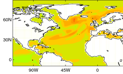
SST sdv ratio (low/total) FEB (GC3.1)
