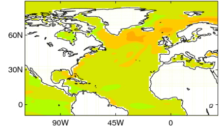
SST sdv ratio (low/total) JUN (GC3.1)
