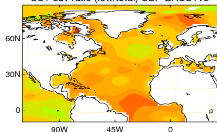
SST sdv ratio (low/total) SEP ERSSTv5
