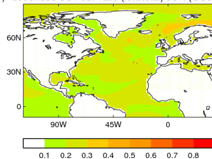
detrended SST sdv ratio (low/total) JUN (GC3.1)
