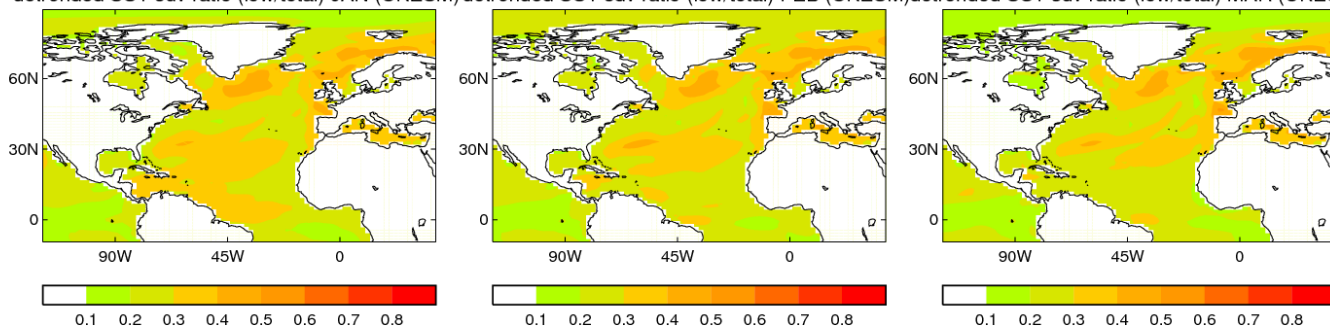
detrended SST sdv ratio (low/total) APR (UKESM)detrended SST sdv ratio (low/total) MAY (UKESM)detrended SST sdv ratio (low/total) JUN (UKESM)
