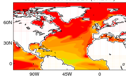
detrended SST sdv DEC (UKESM)
