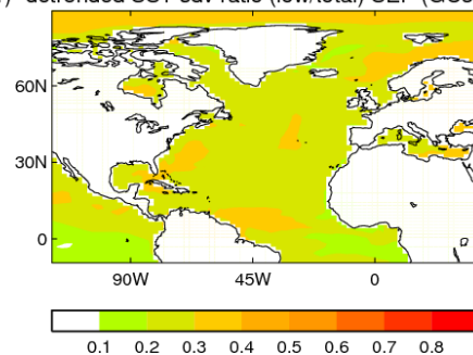
detrended SST sdv ratio (low/total) SEP (GC3.1)
