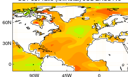
SST sdv ratio (low/total) JUL ERSSTv5
