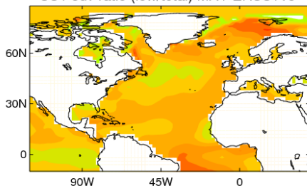
SST sdv ratio (low/total) MAY ERSSTv5
