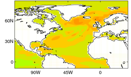
SST sdv ratio (low/total) DEC (GC3.1)
