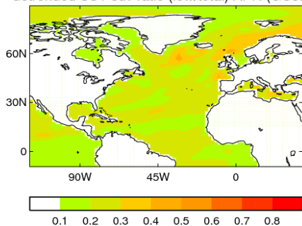
detrended SST sdv ratio (low/total) APR (GC3.1)
