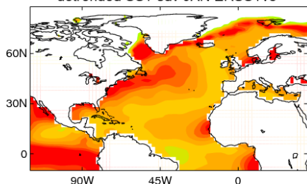
detrended SST sdv JAN ERSSTv5
