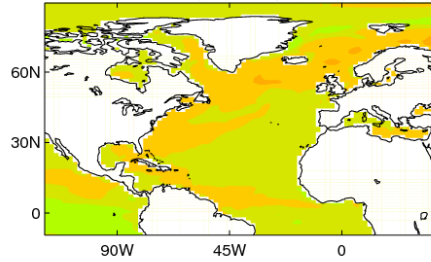
SST sdv ratio (low/total) AUG (GC3.1)
