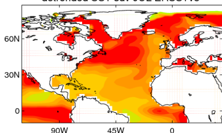
detrended SST sdv JUL ERSSTv5
