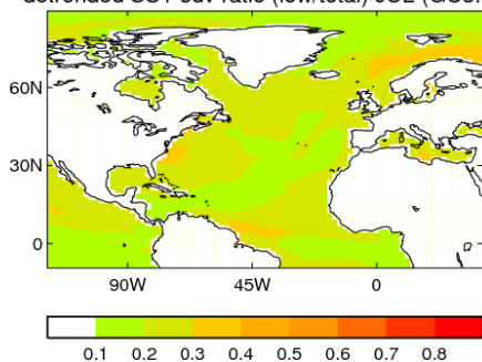
detrended SST sdv ratio (low/total) JUL (GC3.1)
