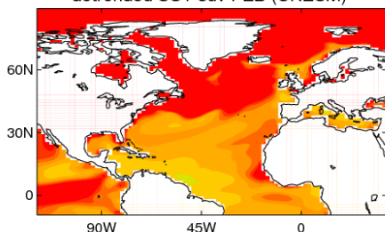
detrended SST sdv FEB (UKESM)
