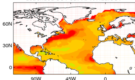
detrended SST sdv APR HadISST
