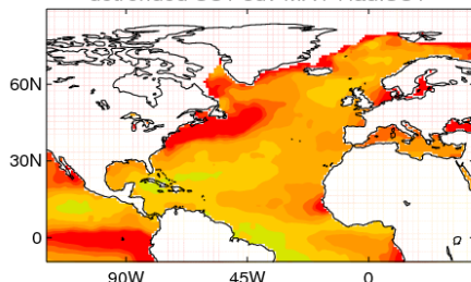
detrended SST sdv MAY HadISST
