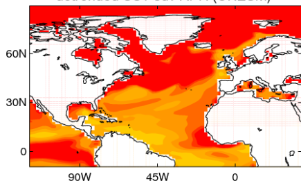
detrended SST sdv APR (UKESM)
