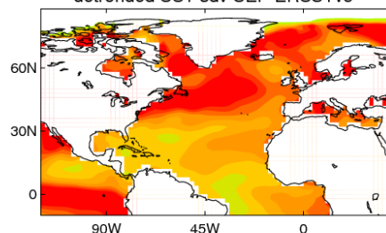
detrended SST sdv SEP ERSSTv5
