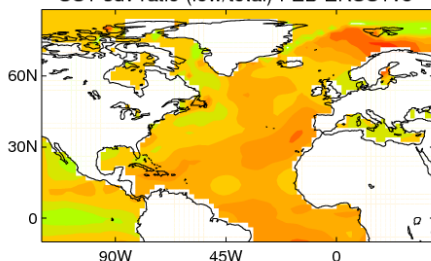
SST sdv ratio (low/total) FEB ERSSTv5
