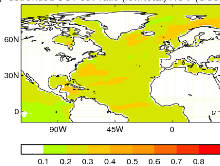
detrended SST sdv ratio (low/total) NOV (GC3.1)
