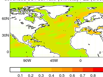
detrended SST sdv ratio (low/total) FEB (GC3.1)
