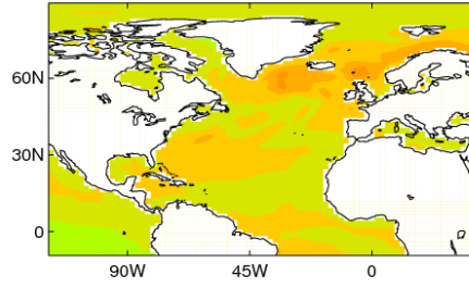
SST sdv ratio (low/total) NOV (GC3.1)
