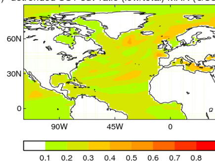
detrended SST sdv ratio (low/total) MAR (GC3.1)
