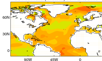
SST sdv ratio (low/total) JUN ERSSTv5
