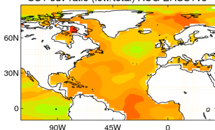
SST sdv ratio (low/total) AUG ERSSTv5
