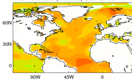
SST sdv ratio (low/total) OCT ERSSTv5
