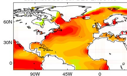
detrended SST sdv DEC ERSSTv5
