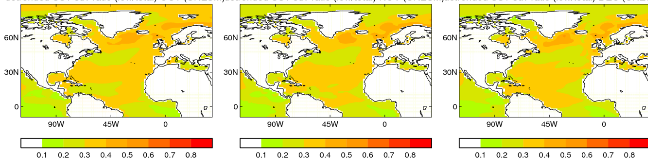
detrended SST sdv ratio (low/total) OCT (UKESM)detrended SST sdv ratio (low/total) NOV (UKESM)detrended SST sdv ratio (low/total) DEC (UKESM)
