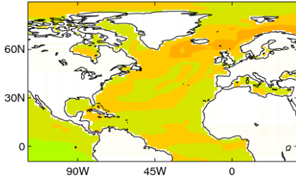
SST sdv ratio (low/total) OCT (GC3.1)
