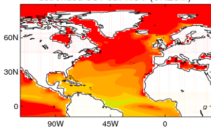
detrended SST sdv NOV (UKESM)
