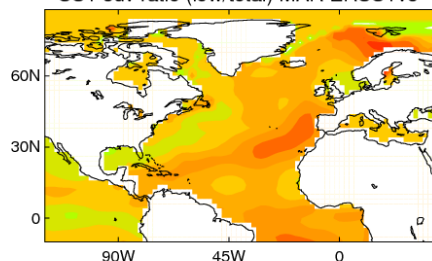
SST sdv ratio (low/total) MAR ERSSTv5
