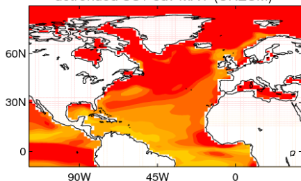
detrended SST sdv MAY (UKESM)
