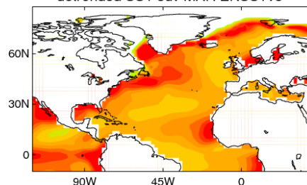
detrended SST sdv MAR ERSSTv5
