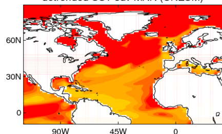
detrended SST sdv MAR (UKESM)
