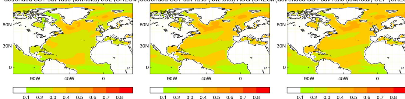
detrended SST sdv ratio (low/total) JUL (UKESM)detrended SST sdv ratio (low/total) AUG (UKESM)detrended SST sdv ratio (low/total) SEP (UKESM)
