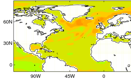
SST sdv ratio (low/total) MAY (GC3.1)
