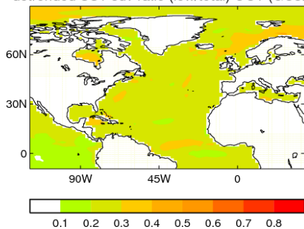
detrended SST sdv ratio (low/total) OCT (GC3.1)
