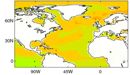
SST sdv ratio (low/total) SEP (GC3.1)
