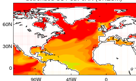
detrended SST sdv JAN (UKESM)
