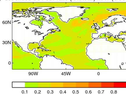
detrended SST sdv ratio (low/total) MAY (GC3.1)
