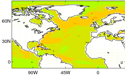
SST sdv ratio (low/total) JUL (GC3.1)
