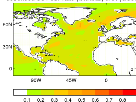
detrended SST sdv ratio (low/total) JAN (GC3.1)
