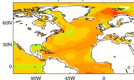
SST sdv ratio (low/total) APR ERSSTv5
