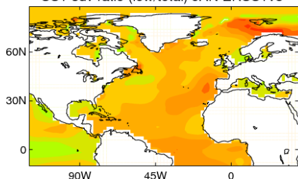
SST sdv ratio (low/total) JAN ERSSTv5
