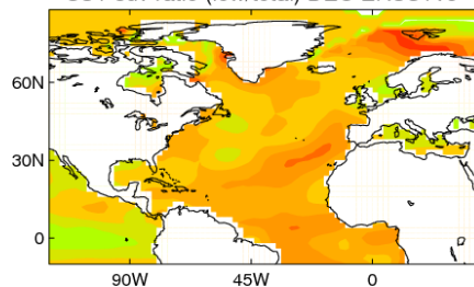
SST sdv ratio (low/total) DEC ERSSTv5
