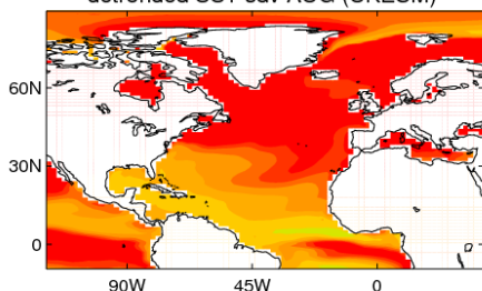
detrended SST sdv AUG (UKESM)
