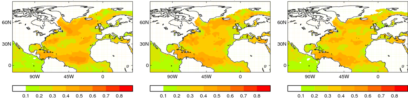
detrended SST sdv ratio (low/total) OCT HadISST detrended SST sdv ratio (low/total) NOV HadISST detrended SST sdv ratio (low/total) DEC HadISST
