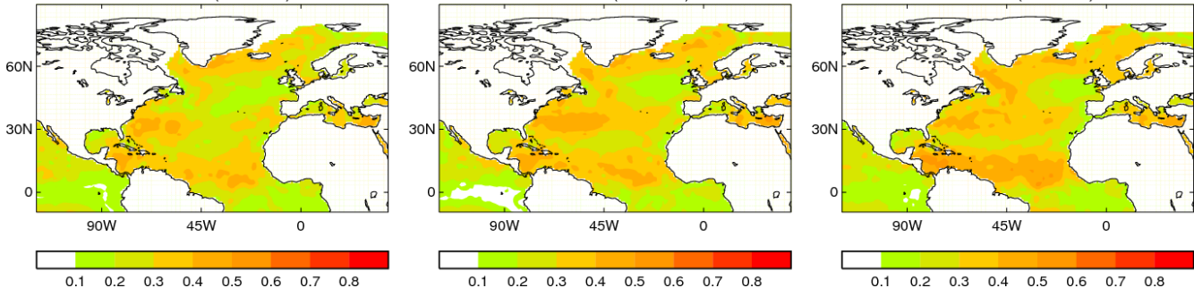
detrended SST sdv ratio (low/total) JUL HadISST detrended SST sdv ratio (low/total) AUG HadISST detrended SST sdv ratio (low/total) SEP HadISST
