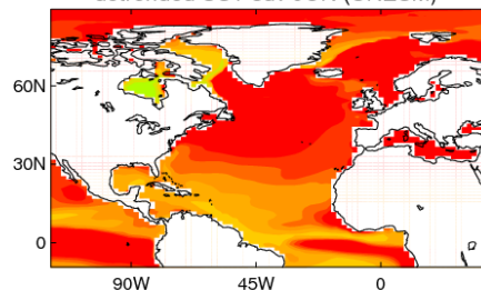
detrended SST sdv JUN (UKESM)
