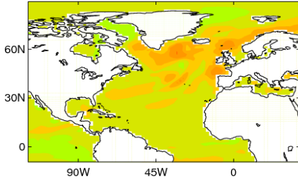
SST sdv ratio (low/total) APR (GC3.1)
