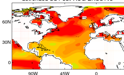
detrended SST sdv AUG ERSSTv5
