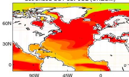
detrended SST sdv JUL (UKESM)
