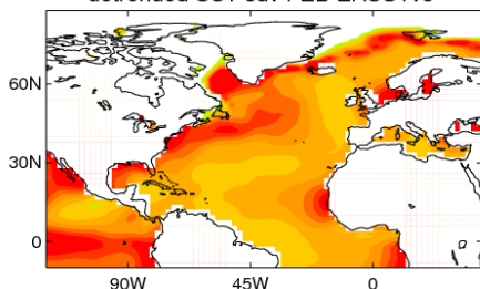
detrended SST sdv FEB ERSSTv5
