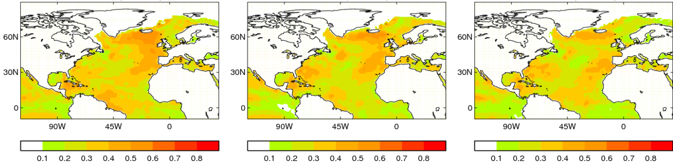
detrended SST sdv ratio (low/total) APR HadISST detrended SST sdv ratio (low/total) MAY HadISST detrended SST sdv ratio (low/total) JUN HadISST
