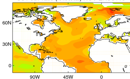
SST sdv ratio (low/total) NOV ERSSTv5
