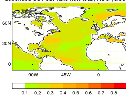
detrended SST sdv ratio (low/total) AUG (GC3.1)
