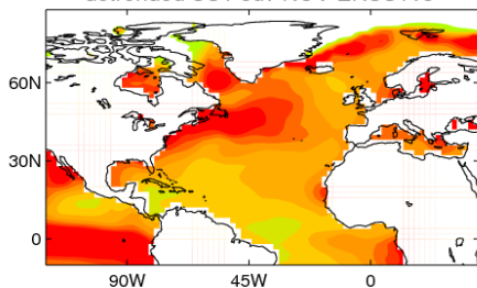
detrended SST sdv NOV ERSSTv5
