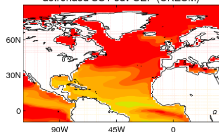
detrended SST sdv SEP (UKESM)
