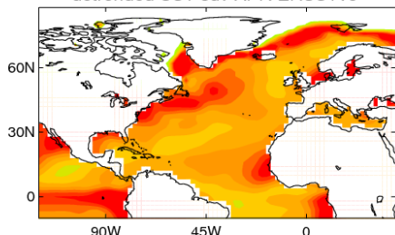
detrended SST sdv APR ERSSTv5
