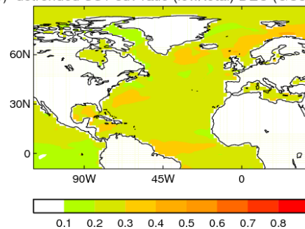
detrended SST sdv ratio (low/total) DEC (GC3.1)
