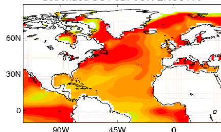
detrended SST sdv JUN ERSSTv5
