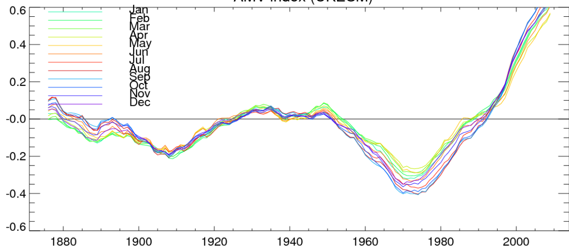
AMV index (UKESM)
