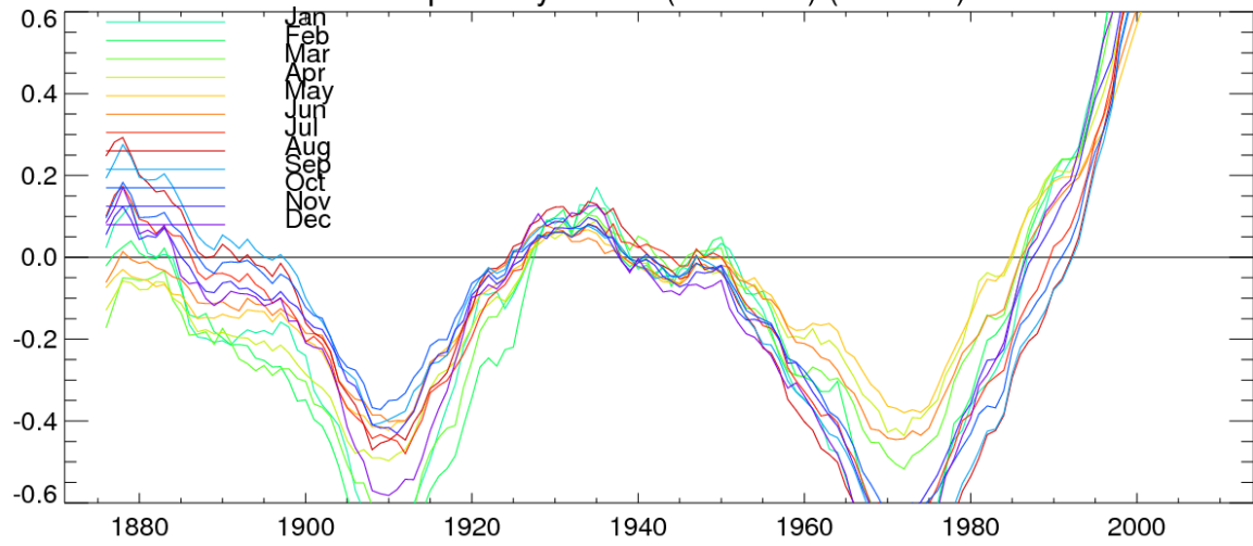
Subpolar Gyre SST (45N-67N) (UKESM)
